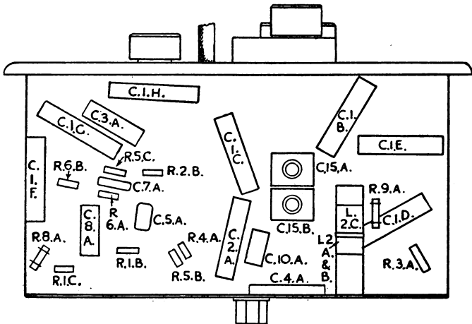
FIG. 10. UNDERSIDE VIEW OF CHASSIS
