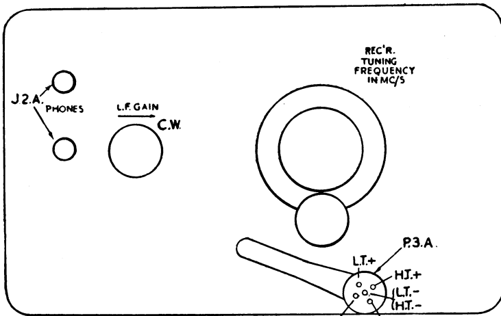
FIG. 7. FRONT VIEW OF RECEIVER PANEL
