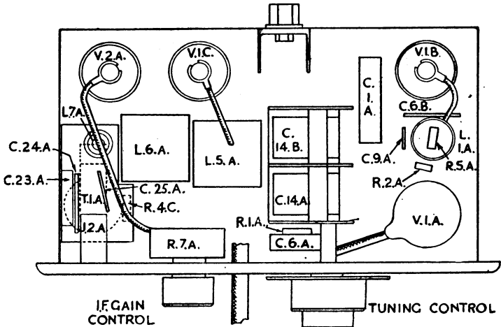
FIG. 9. TOP VIEW OF CHASSIS
