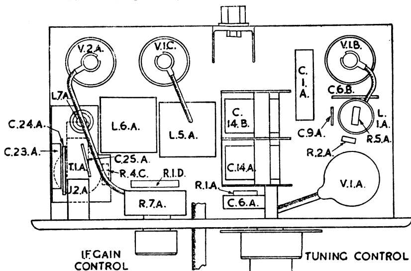
FIG. 3. TOP VIEW OF CHASSIS
